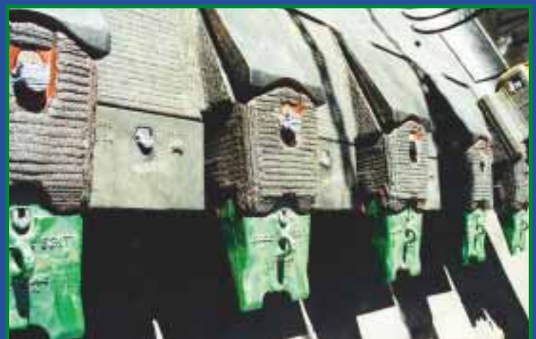
P&H Dragline Bucket Lip Shrouds A.R.M* Hardfaced.
